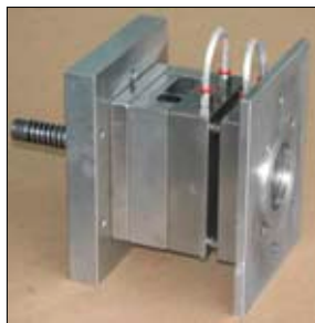
80mm test bar and 60mm short tensile bar
